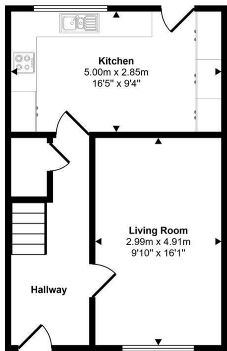
Ground Floor Approx 40 sq m / 426 sq ft
